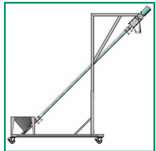
Portable base (fixed or tilting)
